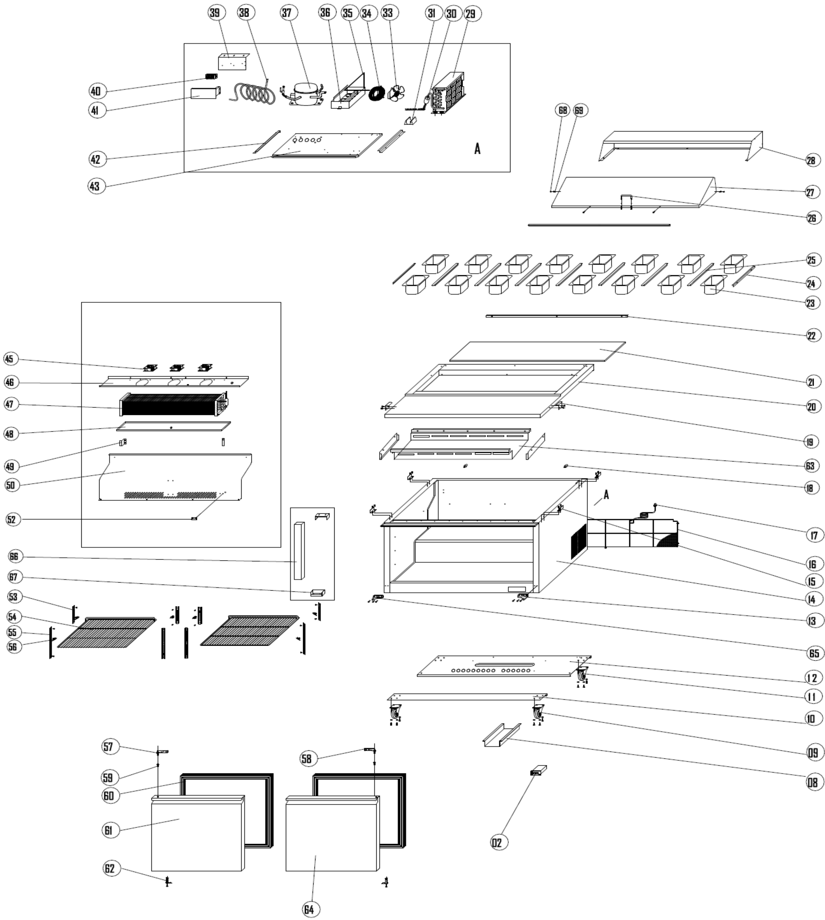
EXPLODE OF KCHST60.16
